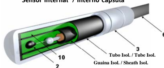
Sensor internal / Interno capsula
